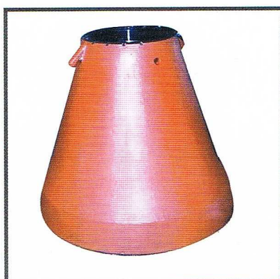
Mantle for Con Crusher (Material : High-Mn Steel)
