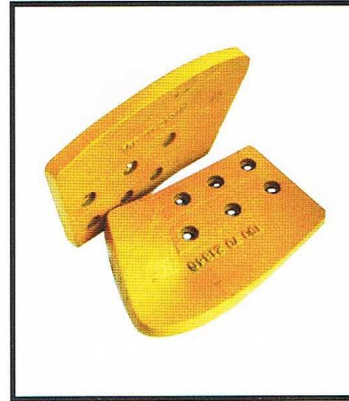
Model: LE70 Part No: 1507021346 / 1507021356 Specification : Thickness=1 3/8"
