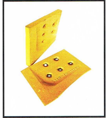
Model: A6 Part No: 1407011170 / 1407011180 Specification : Thickness=1"
