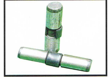
Model: PC 300-5/6 Material: S45C Size: Length=120mm \varnothing 24.5mm
